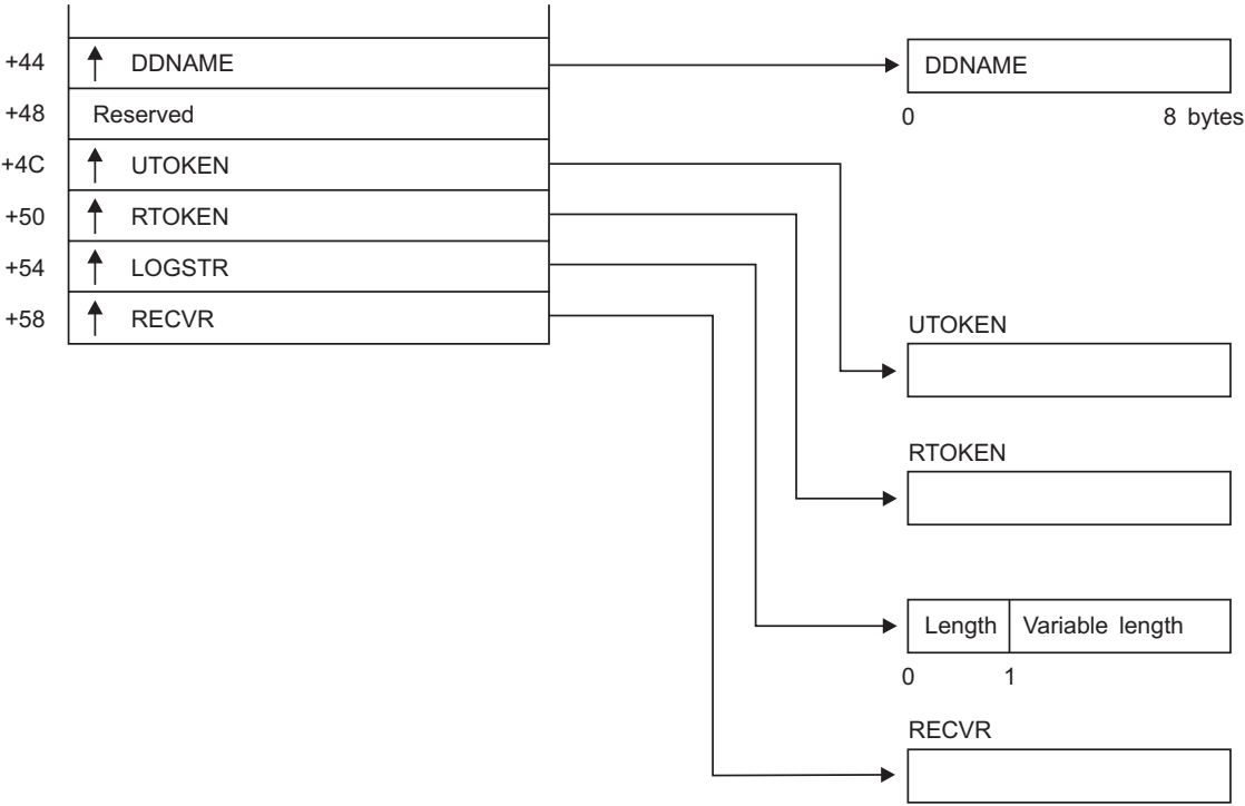
Figure 28. AUTH Service Parameter List (Part 4 of 4)
