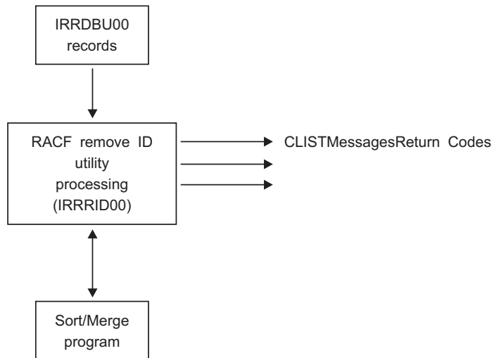
Figure 44. Process Flow for RACF Remove ID Utility
