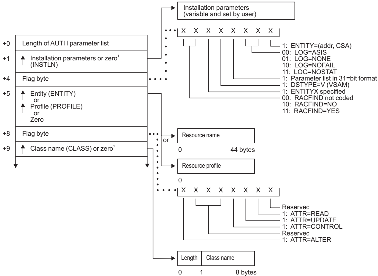
Figure 28. AUTH Service Parameter List (Part 1 of 4)
