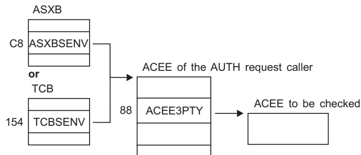
Figure 55. Control Block Overview: ACEEs When Third-Party AUTH Request Is Used
