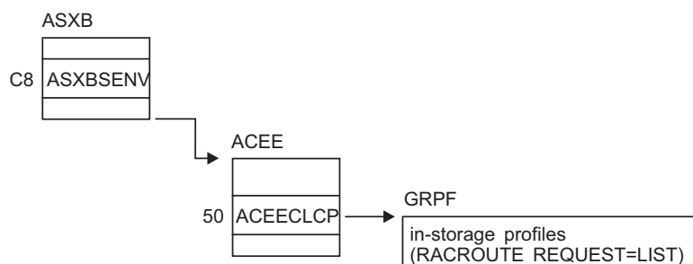
Figure 53. Control Block Overview: ACEE in a Single-User Address Space
