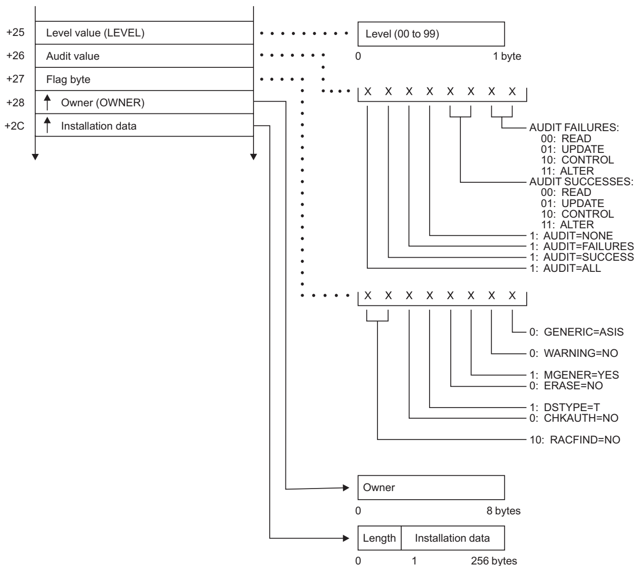
Figure 29. DEFINE Service Parameter List (Part 3 of 6)
