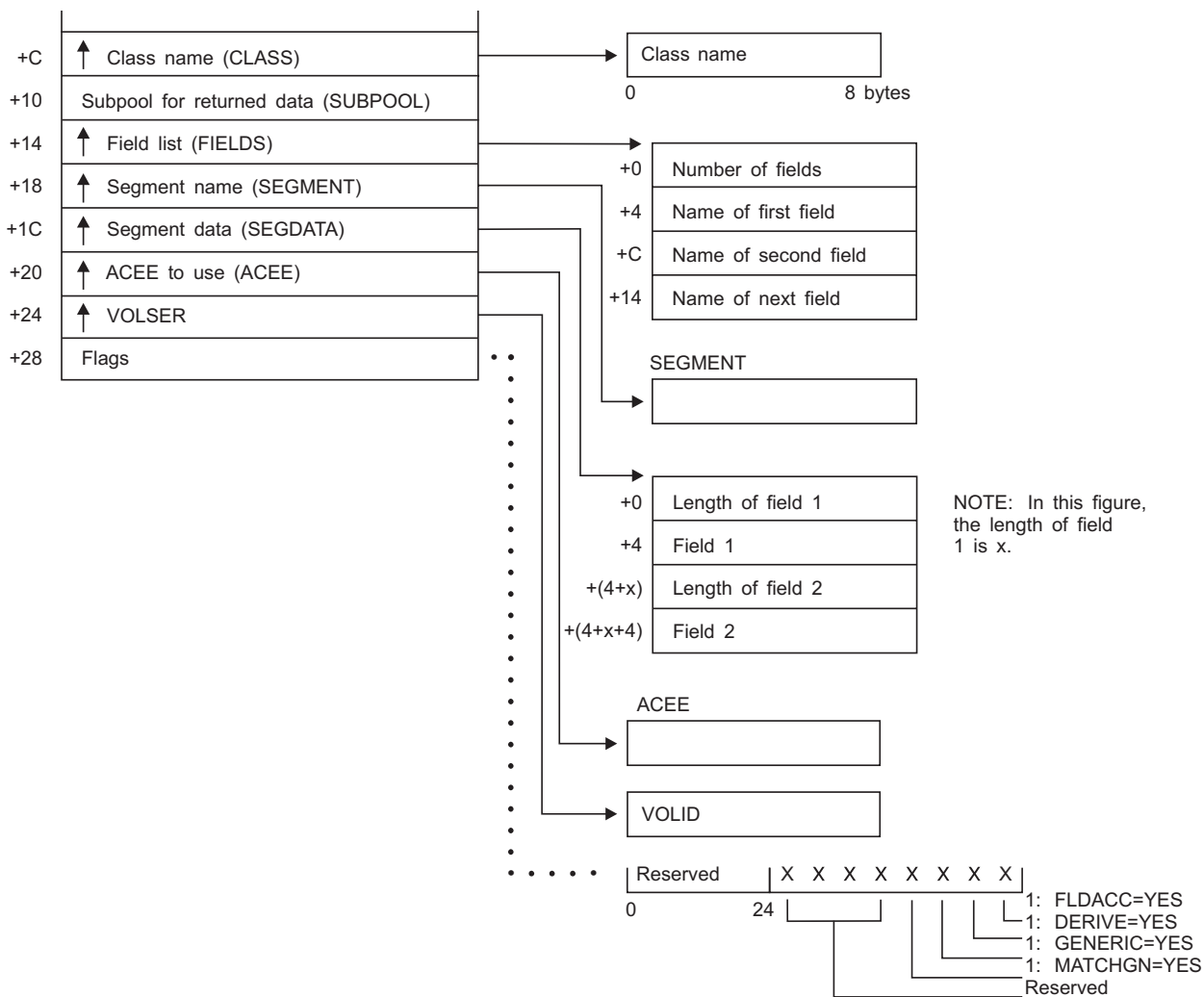
Figure 31. EXTRACT Service Parameter List (Part 3 of 3)
