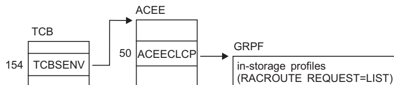
Figure 54. Control Block Overview: ACEE in a Multiple-User Address Space
