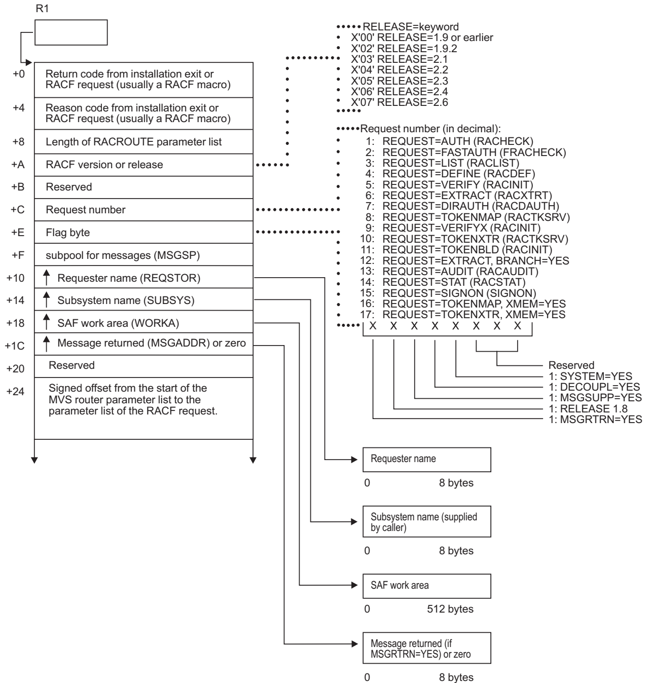
Figure 26. RACROUTE Parameter List (Part 1 of 2)
