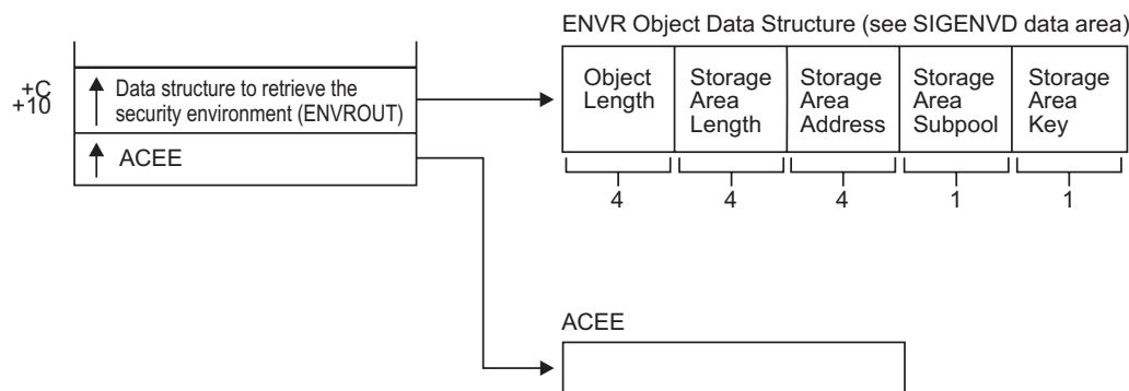
Figure 31. EXTRACT Service Parameter List (Part 2 of 3)
