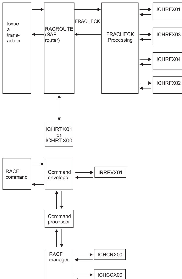
Figure 42. Process Flow for RACF Installation Exits (Part 2 of 2)
