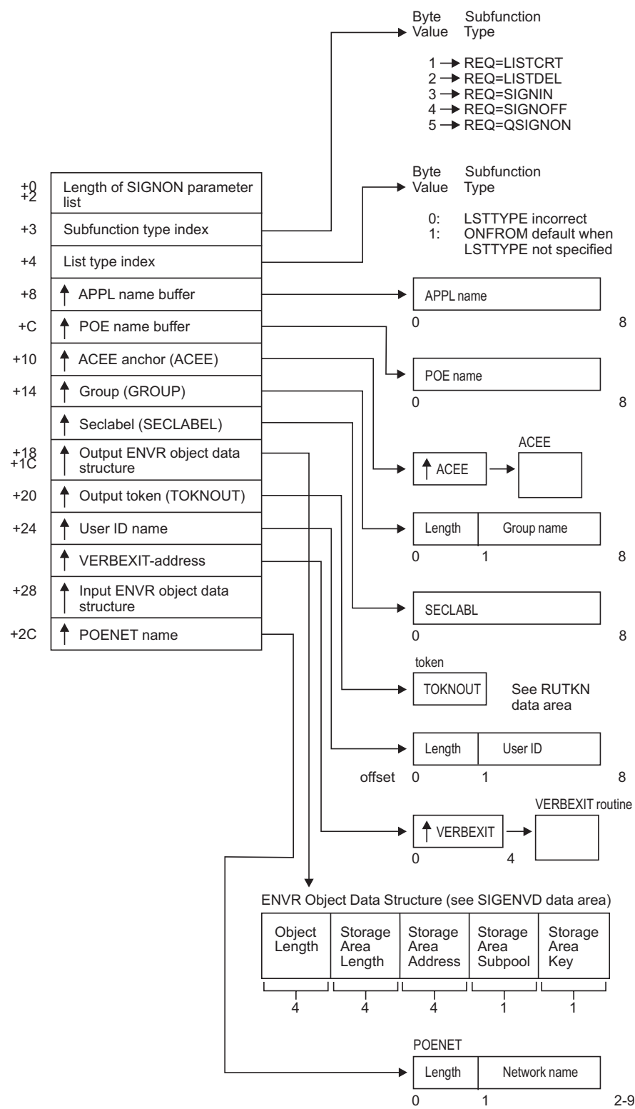
Figure 34. SIGNON Service Parameter List
