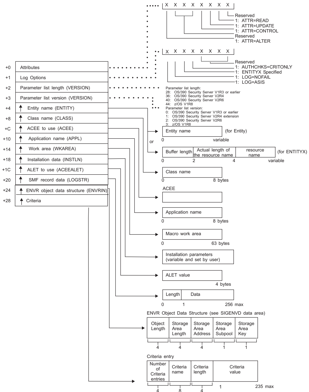
Figure 32. FASTAUTH Service Parameter List
