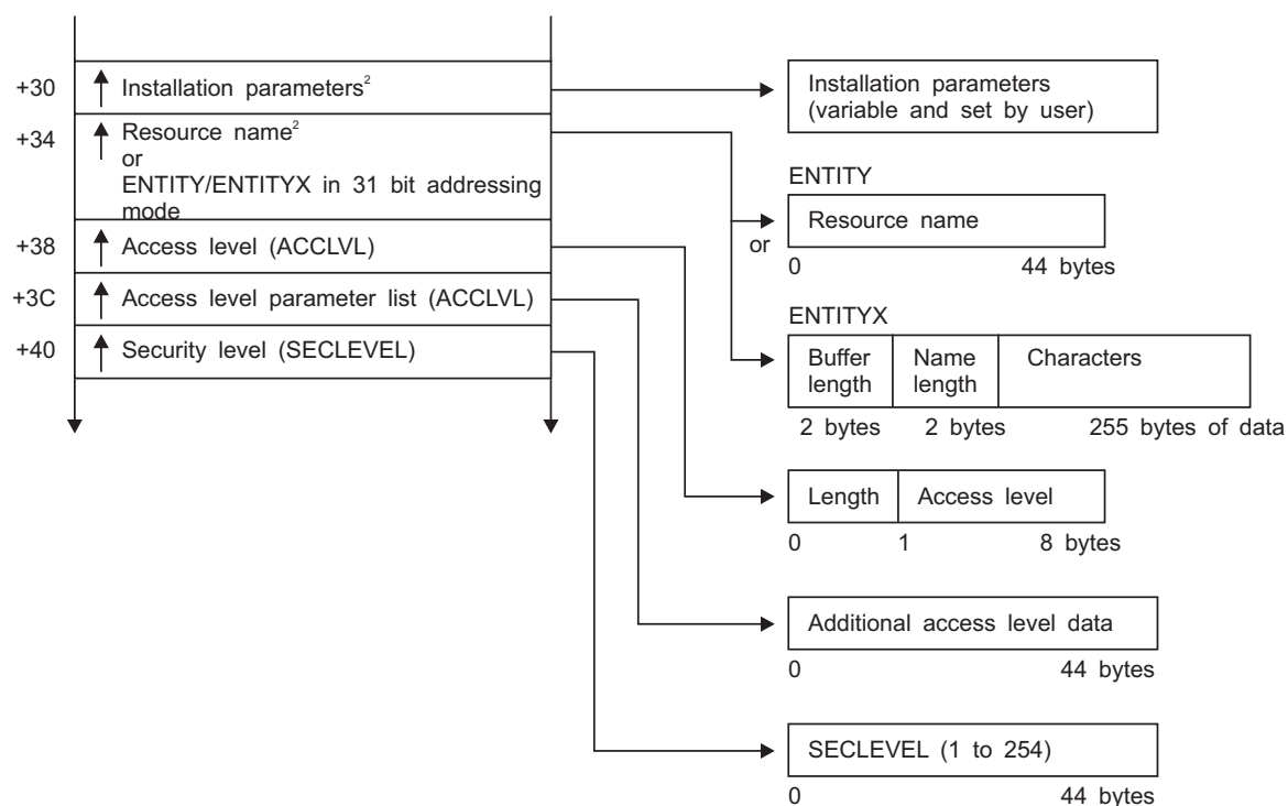
Figure 29. DEFINE Service Parameter List (Part 4 of 6)
