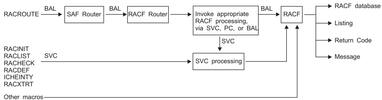
Figure 41. Process Flow for RACF Macros
