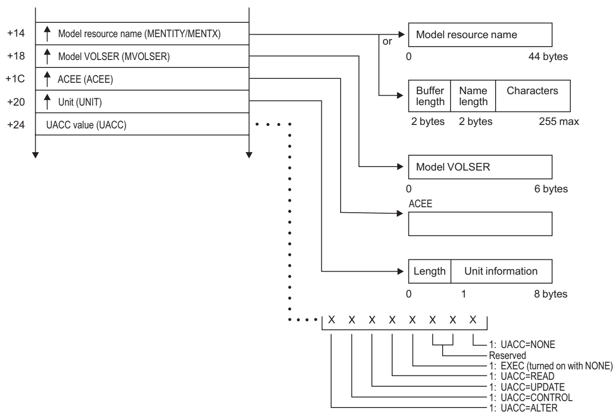
Figure 29. DEFINE Service Parameter List (Part 2 of 6)
