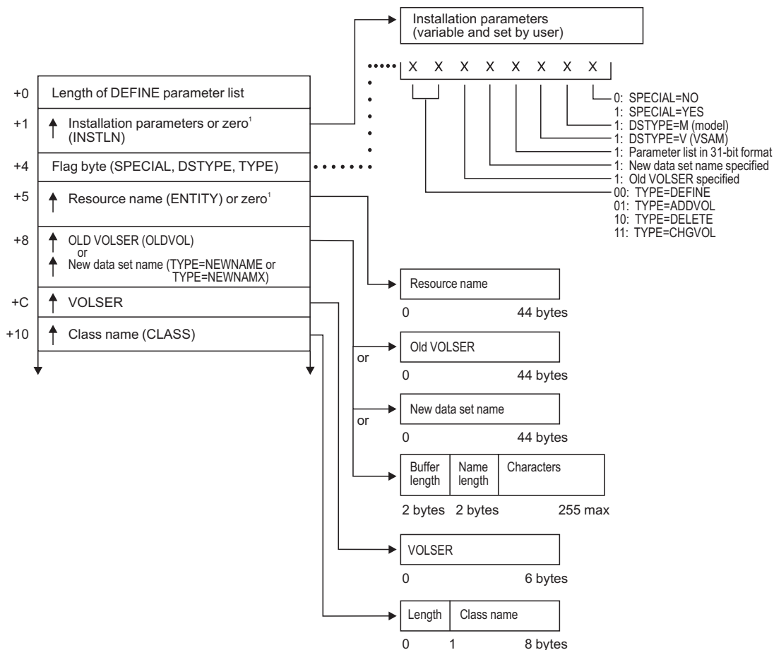
Figure 29. DEFINE Service Parameter List (Part 1 of 6)
