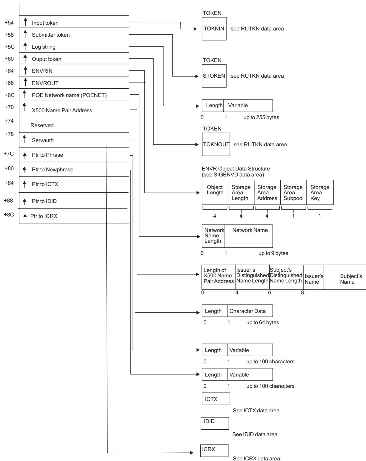
Figure 37. VERIFY/VERIFYX Service Parameter List (Part 4 of 4)
