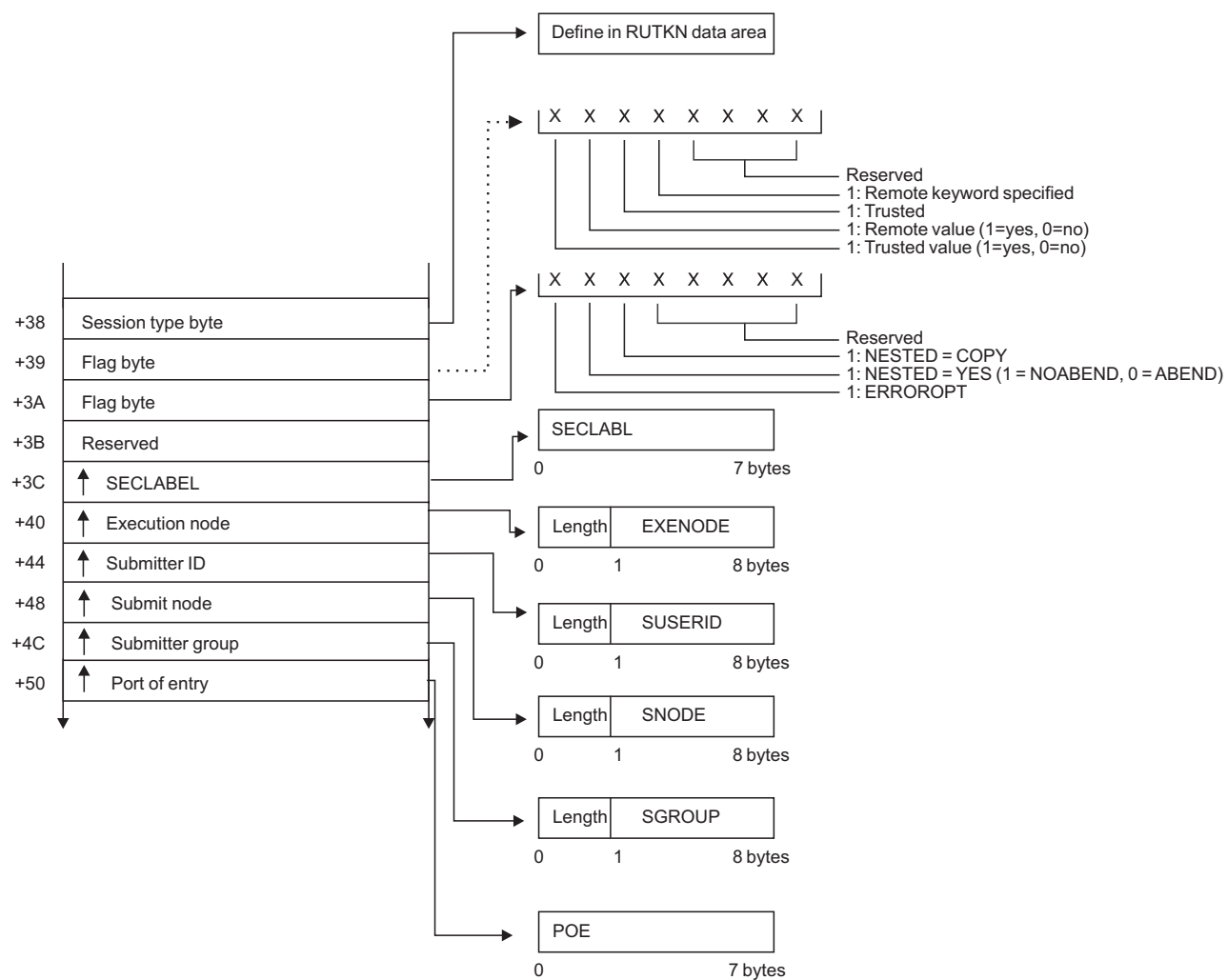
Figure 37. VERIFY/VERIFYX Service Parameter List (Part 3 of 4)
